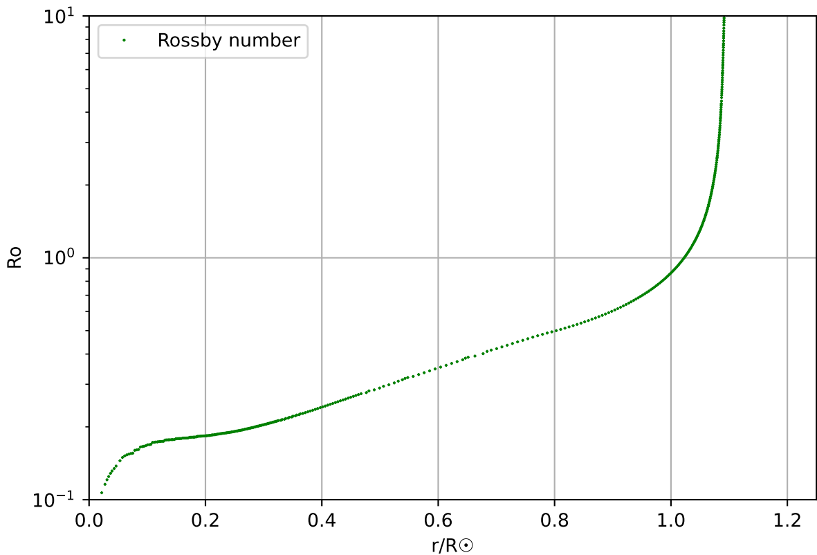
Rossby number, profile 159, age 7.2 \times 10^9
